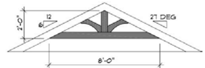
Straight Accent Truss "D" $600
