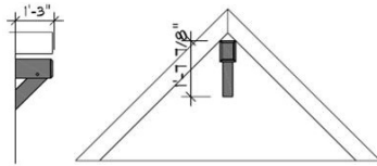
Corbel "B" $250 (no vents when corbels are installed)
