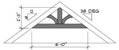
Straight Accent Truss "F" $600
